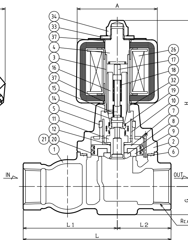
DIMENSIONS (mm)
