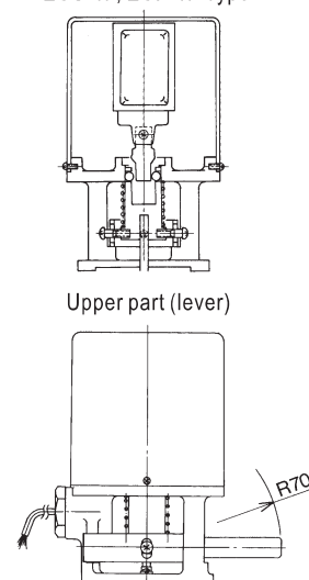
ECS-1P, ECF-1P Type
