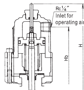
Gland of COS/CCS-1H Type
