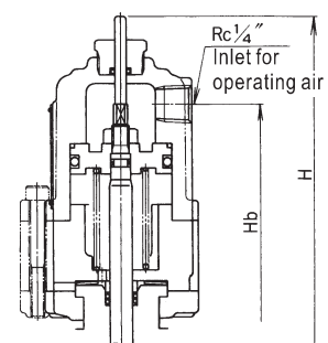
Drive unit of CCF-1, 1H Type
