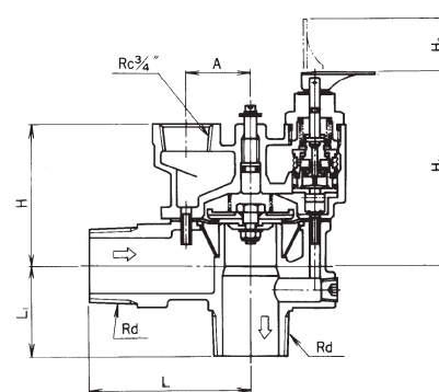
LP-8ARN Type
