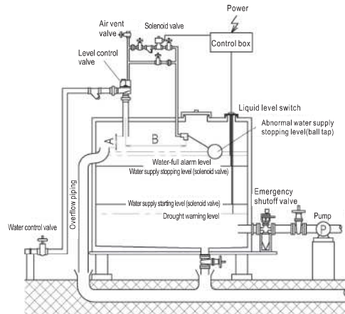
Fig.2: Angular type
