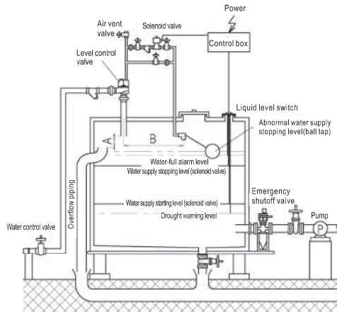
Fig.2: Angular type
