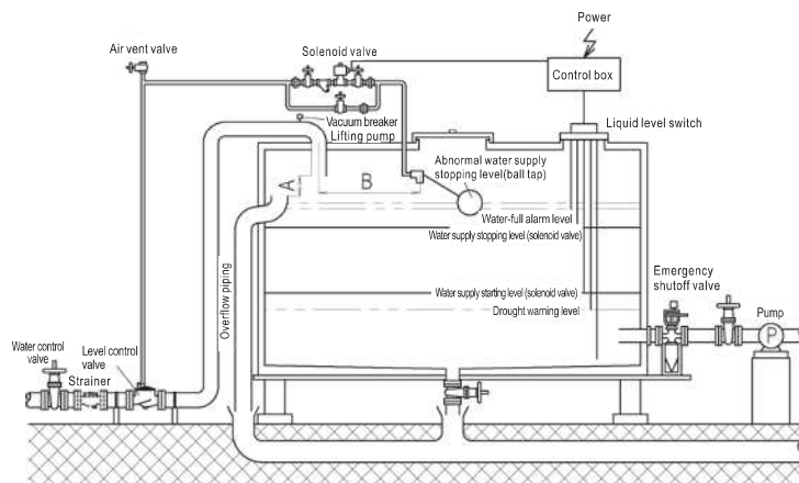
Fig.1: Straight type
