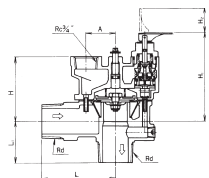
LP-8ARN Type
