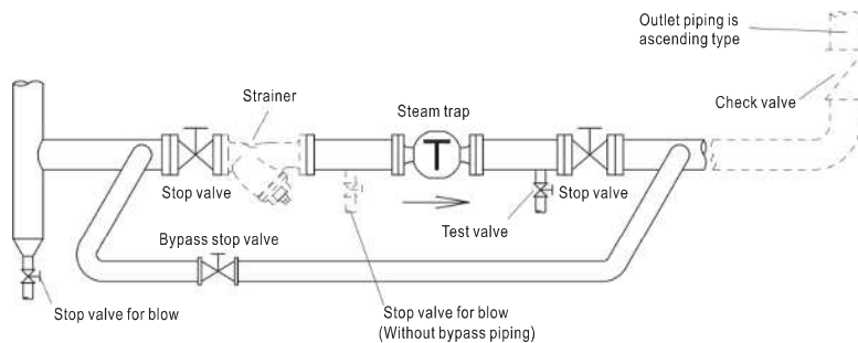
Fig. 1 Piping example
