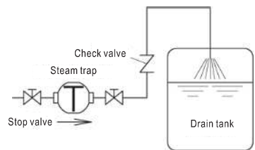
Fig.6 Waterspout Piping Example
