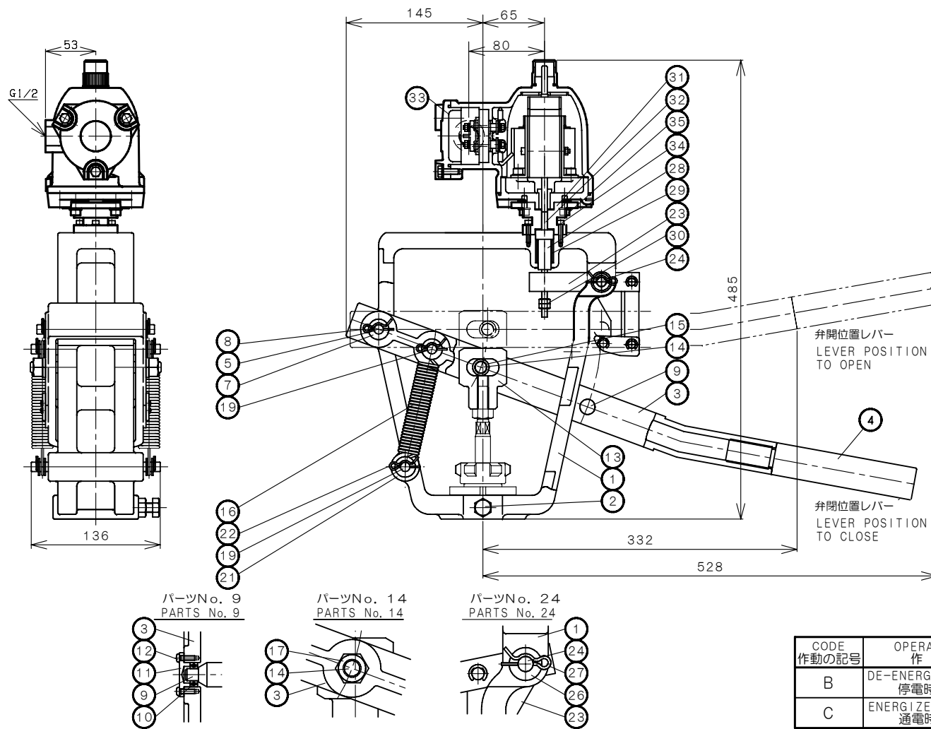
DE-ENERGIZED CLOSE TYPE STOPPER (RESET MANUALLY FOR OPEN)
