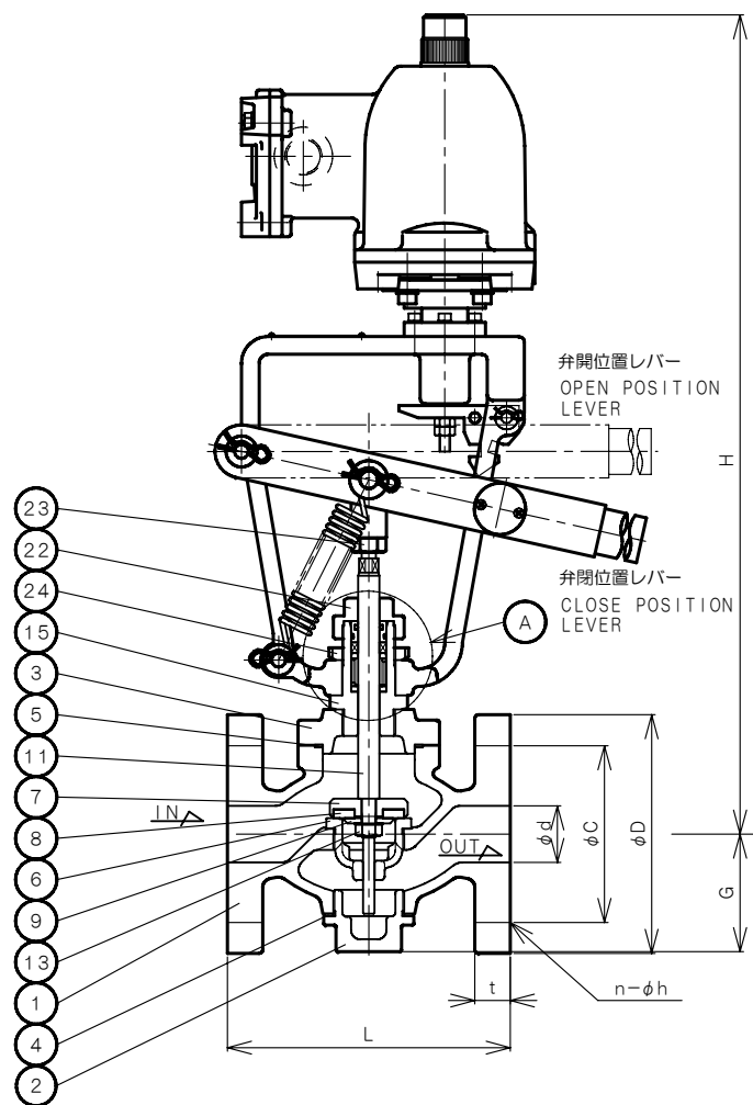
DIMENSIONS (mm) FLANGE CODE: JIS 10K FF
