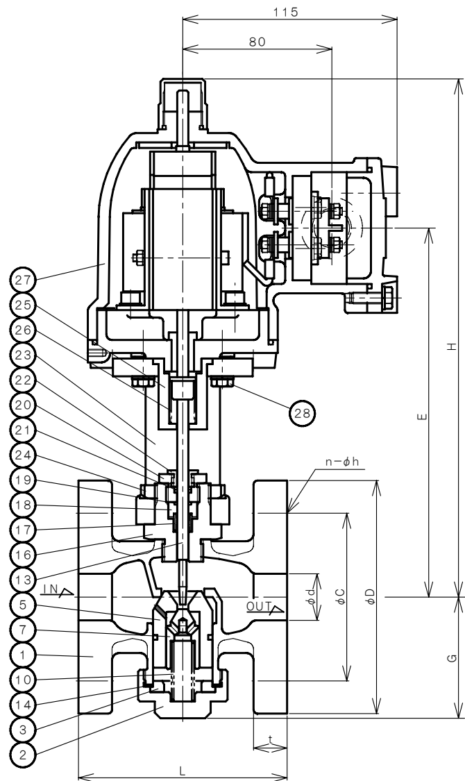
DIMENSIONS (mm) FLANGE CODE: JIS 10K FF
