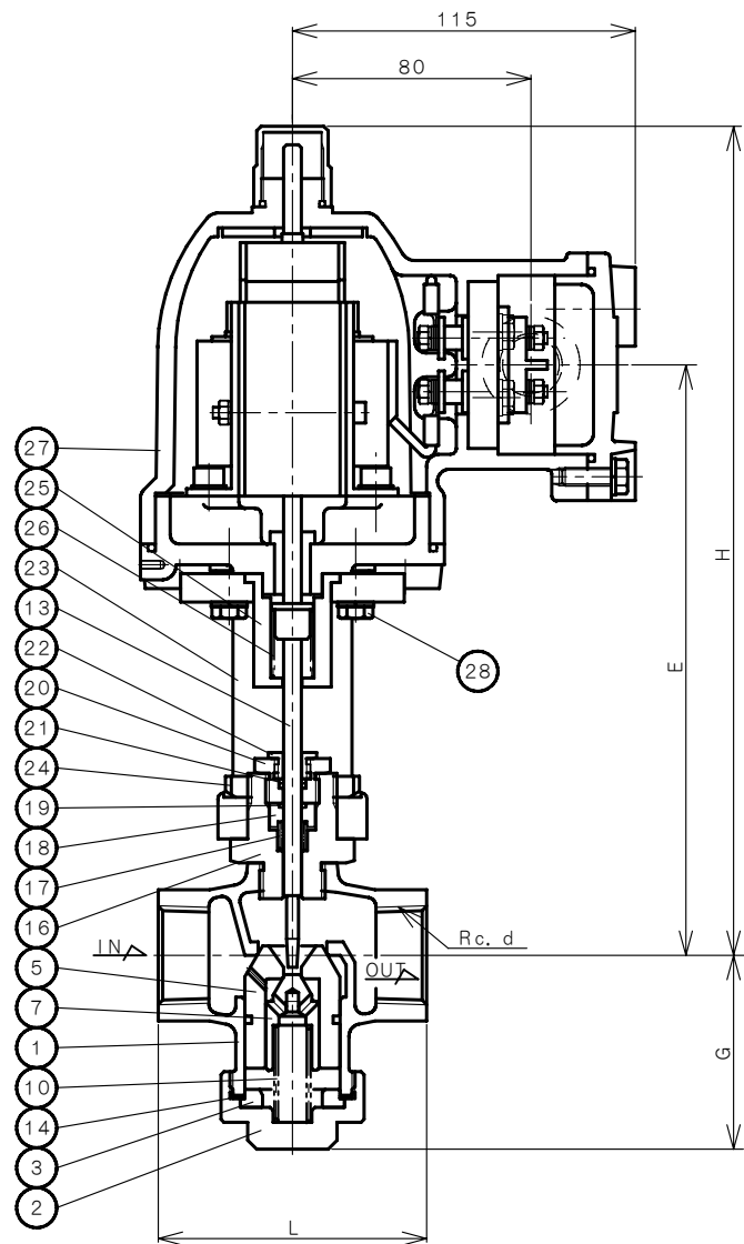
DIMENSIONS (mm)
