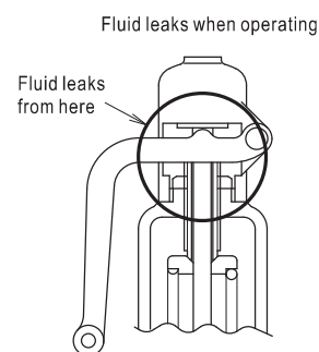
Open type lever structure
