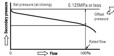
Spring range [H]: Size ≤100mm: 0.3~0.7MPa Size 125mm, 150mm: 0.3~0.5MPa
