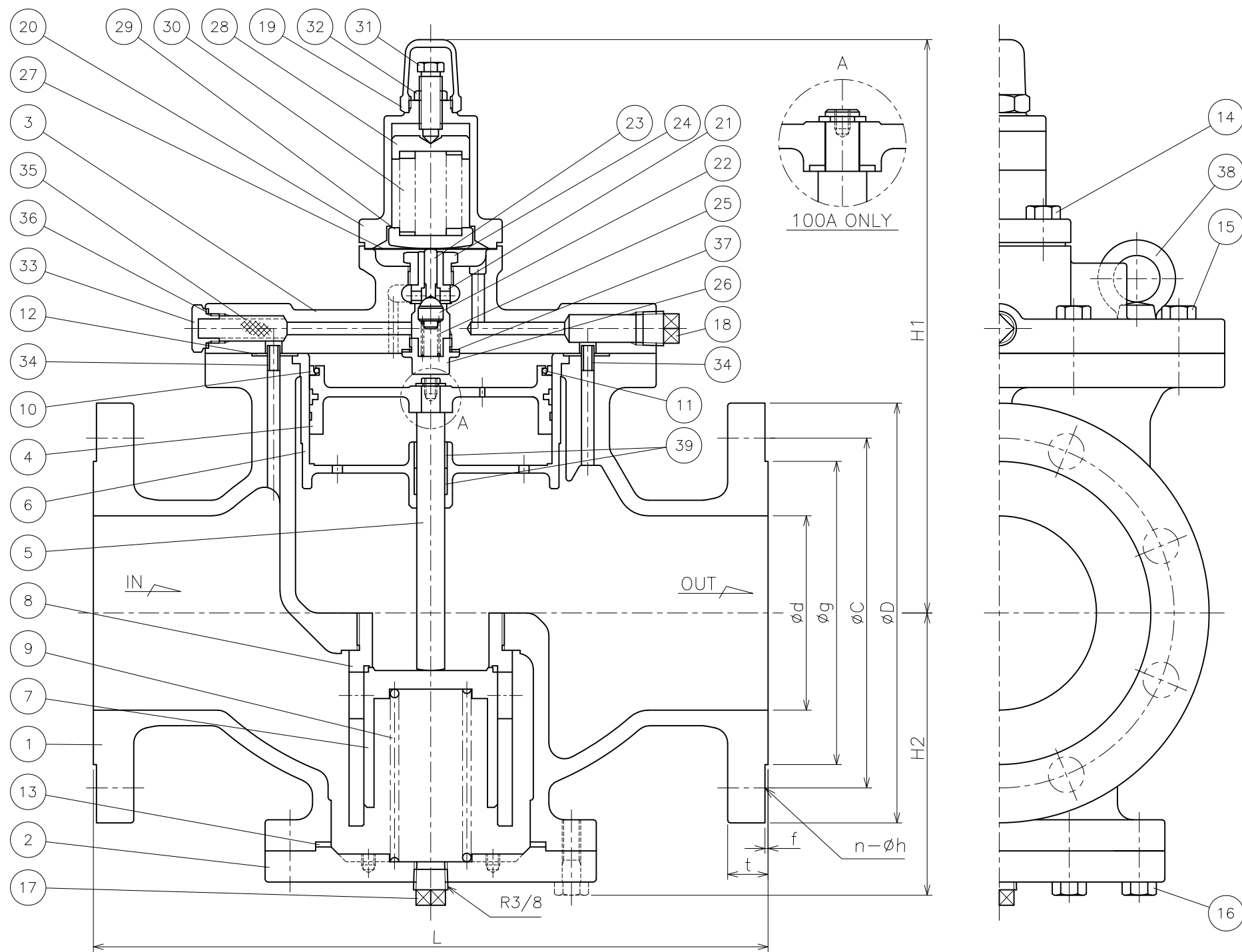
DIMENSIONS (mm)
