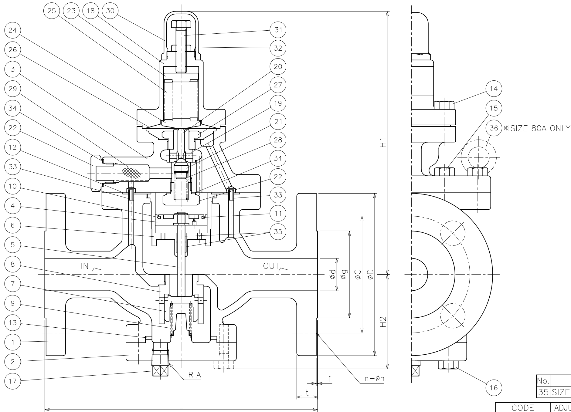
DIMENSIONS (mm)
