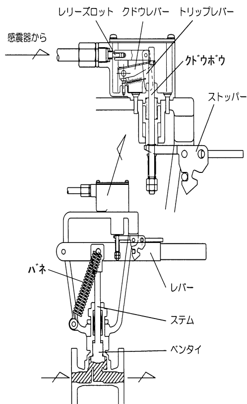
図１－５：作動図＜弁開状態＞
