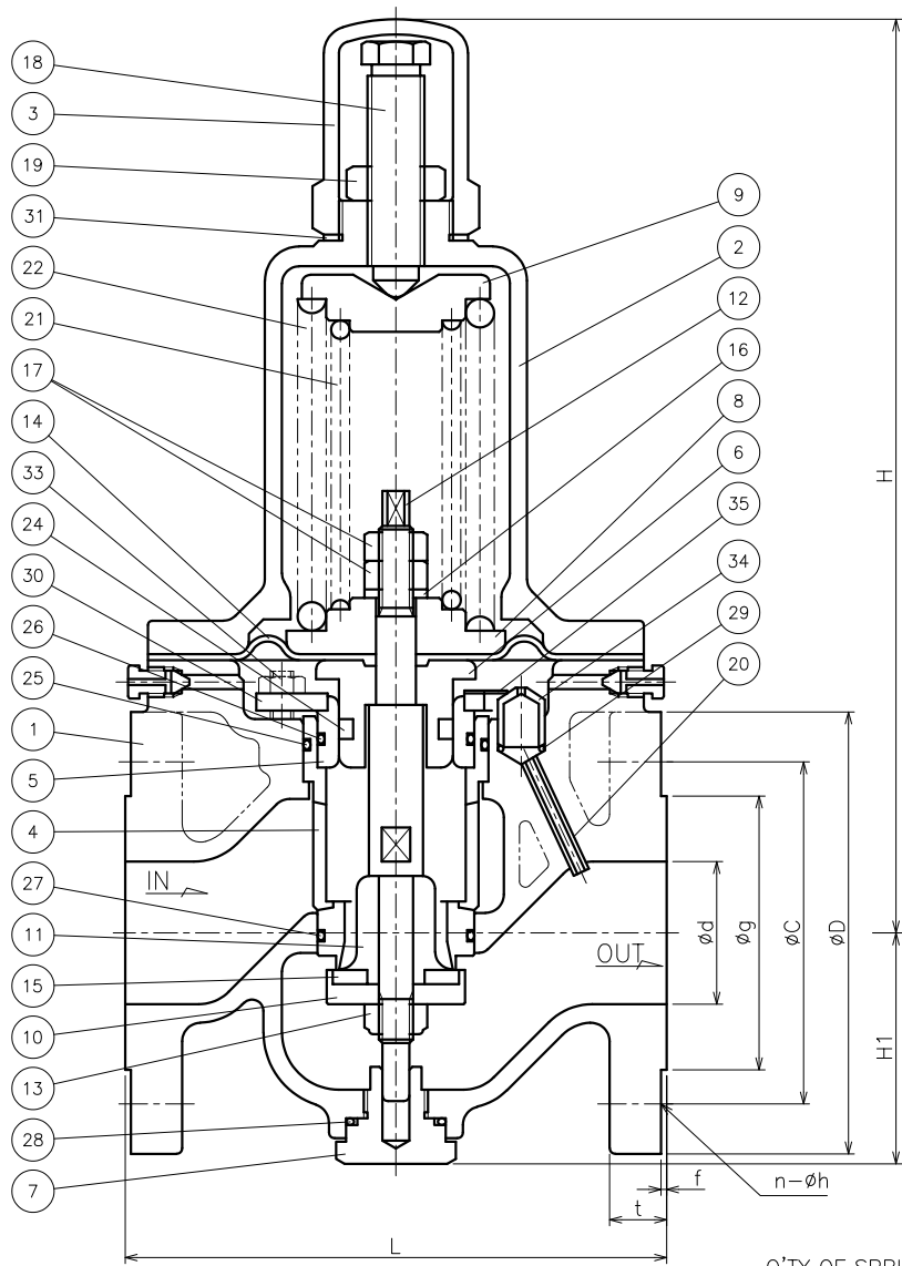
DIMENSIONS (mm) FLANGE CODE: JIS 10K
