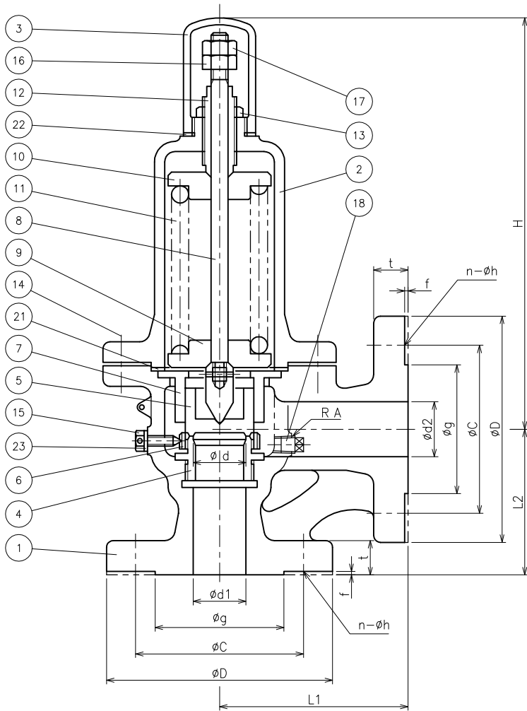
DIMENSIONS ( mm )
