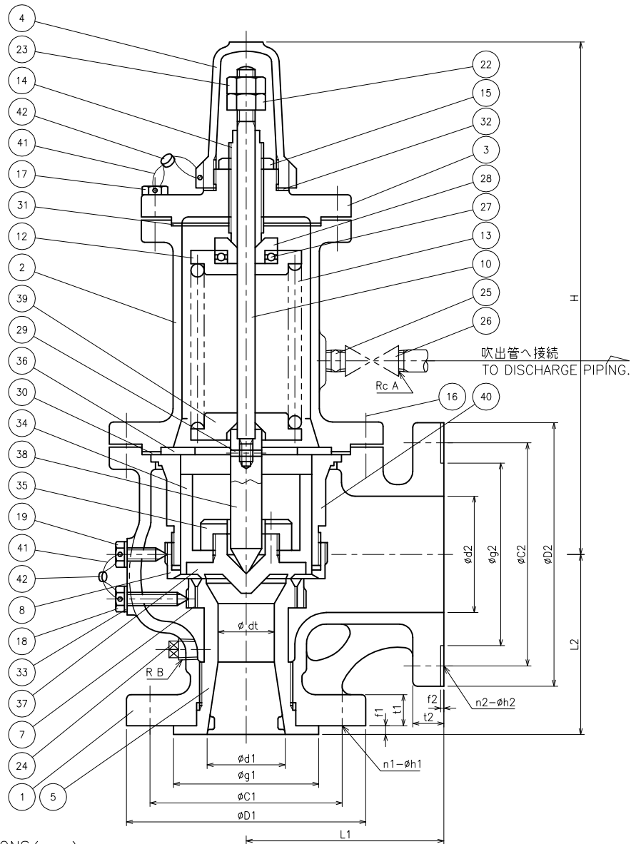
DIMENSIONS (mm)
