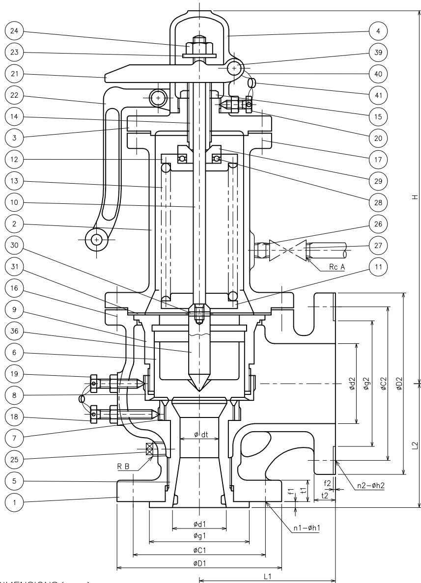
DIMENSIONS (mm)
