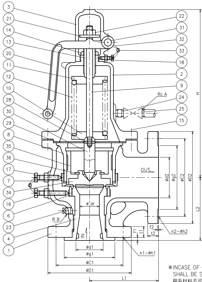
DIMENSIONS (mm)
