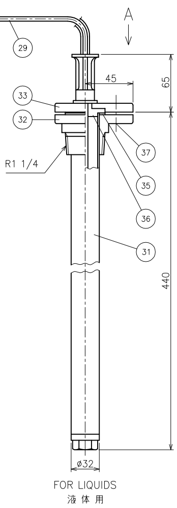
DIMENSIONS (mm)
