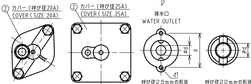
寸法表 (DIMENSION) (mm)
