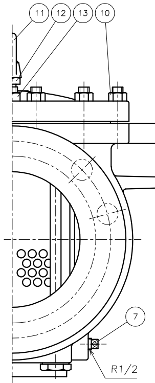
DIMENSIONS (mm) FLANGE CODE: JIS 10K
