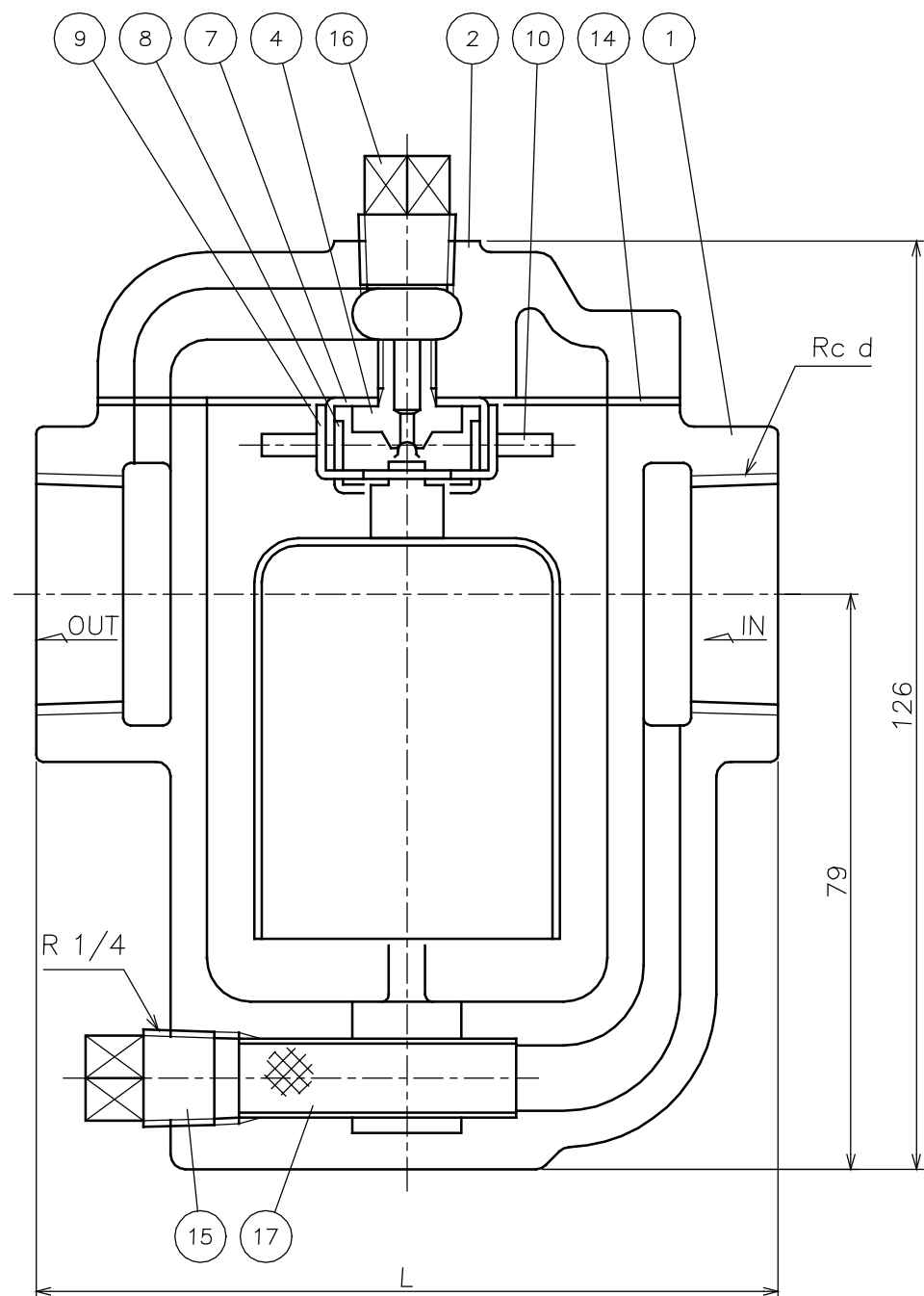
DIMENSIONS (mm)
