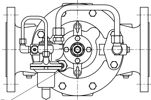
PLANE FIG.
