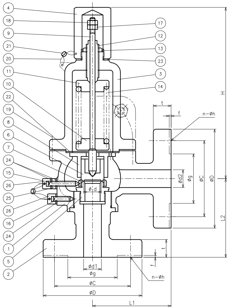
DIMENSIONS (mm)
