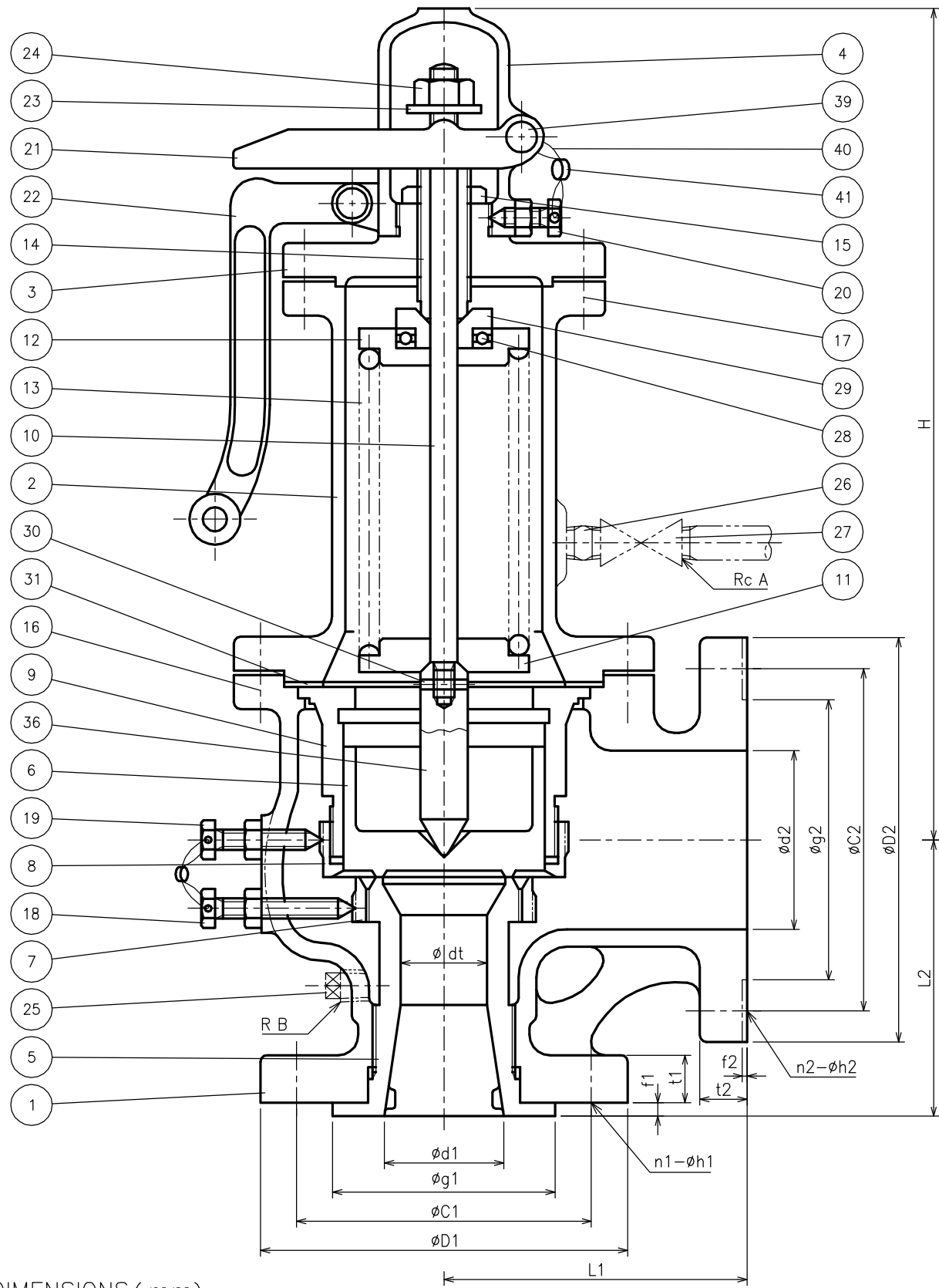
DIMENSIONS (mm)
