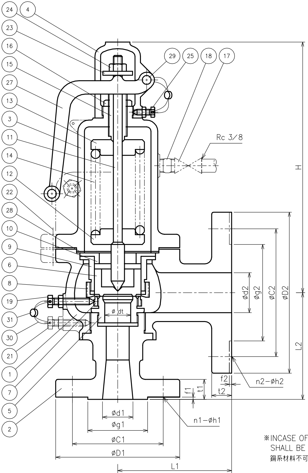
DIMENSIONS (mm)
