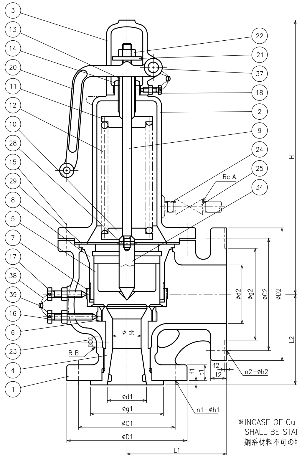
DIMENSIONS (mm)
