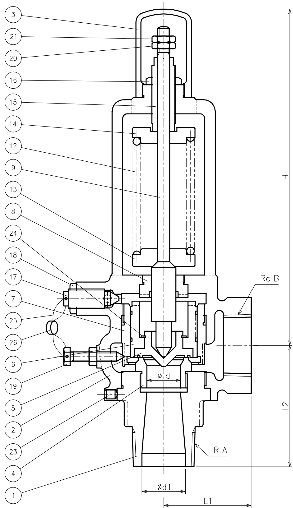
DIMENSIONS (mm)
