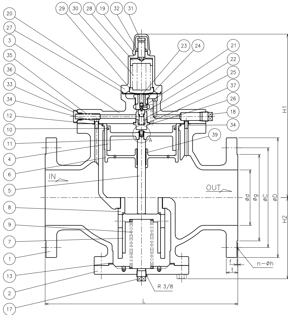
DIMENSIONS ( mm )
