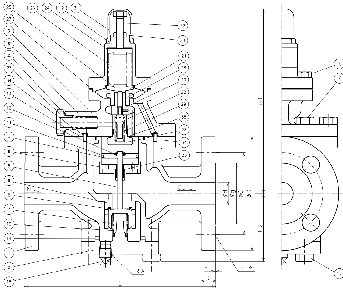
DIMENSIONS (mm)
