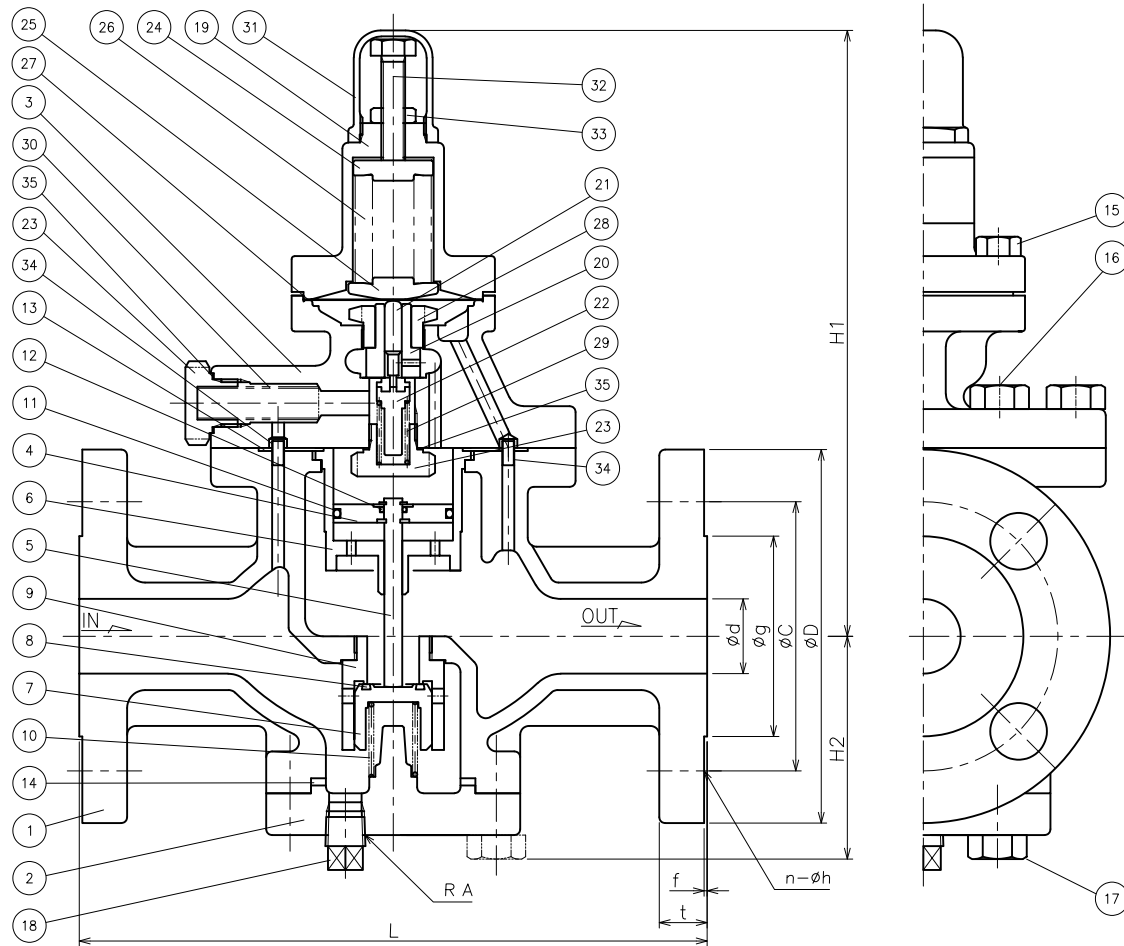
DIMENSIONS (mm)
