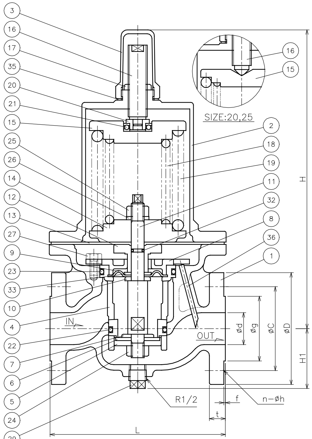
DIMENSIONS (mm)
