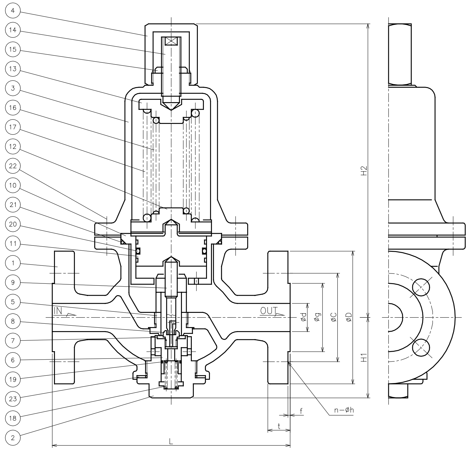
DIMENSIONS (mm)
