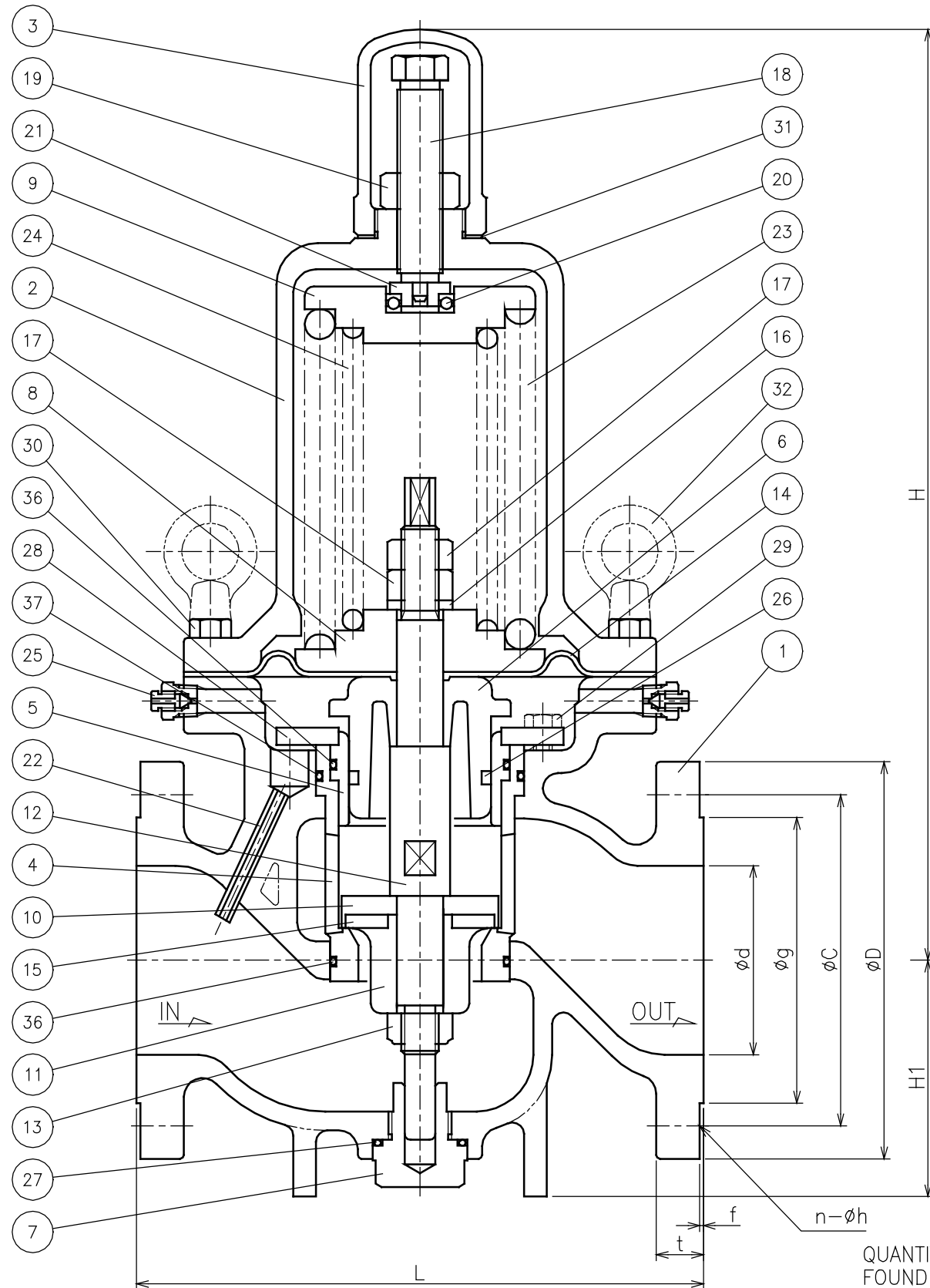
DIMENSIONS ( mm )
