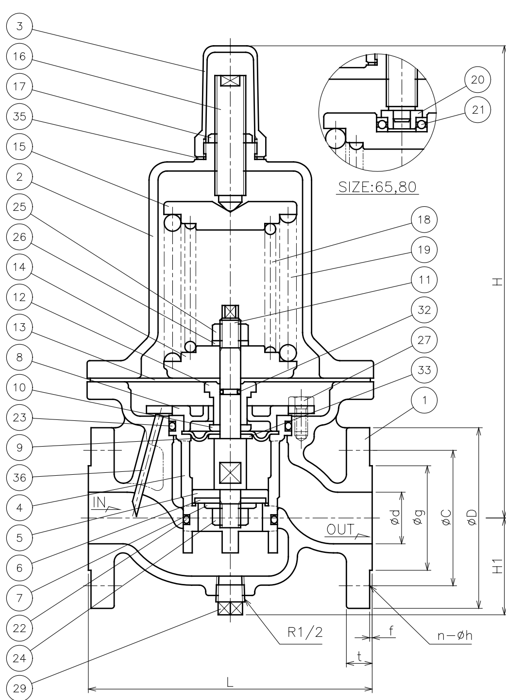
DIMENSIONS (mm)
