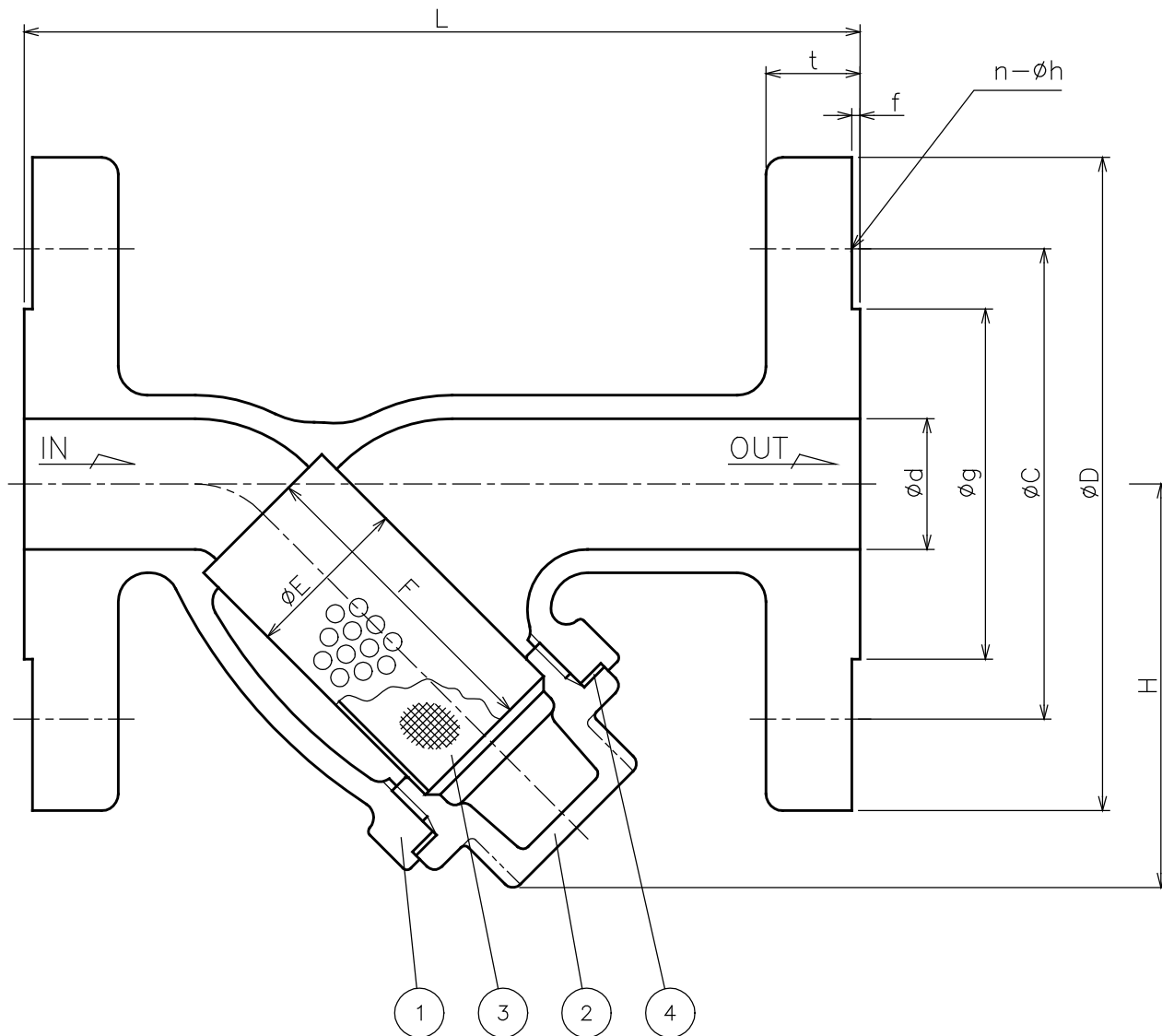
DIMENSIONS (mm) FLANGE CODE: JIS 10K
