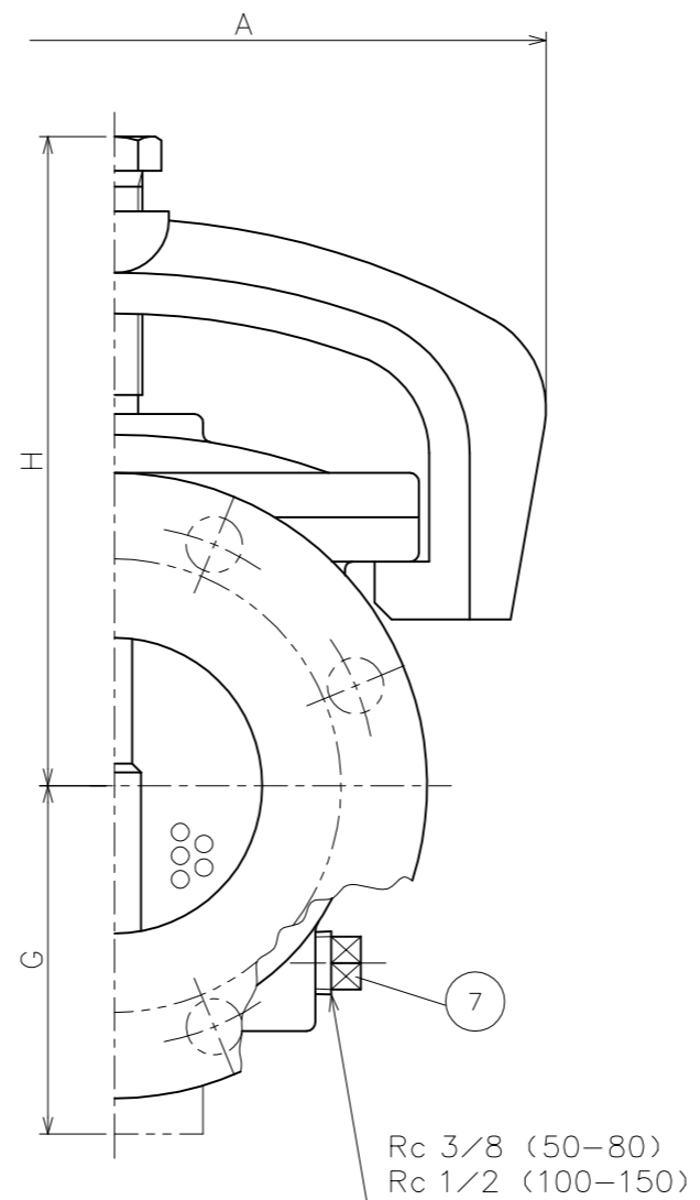
DIMENSIONS (mm) FLANGE CODE: JIS 10K
