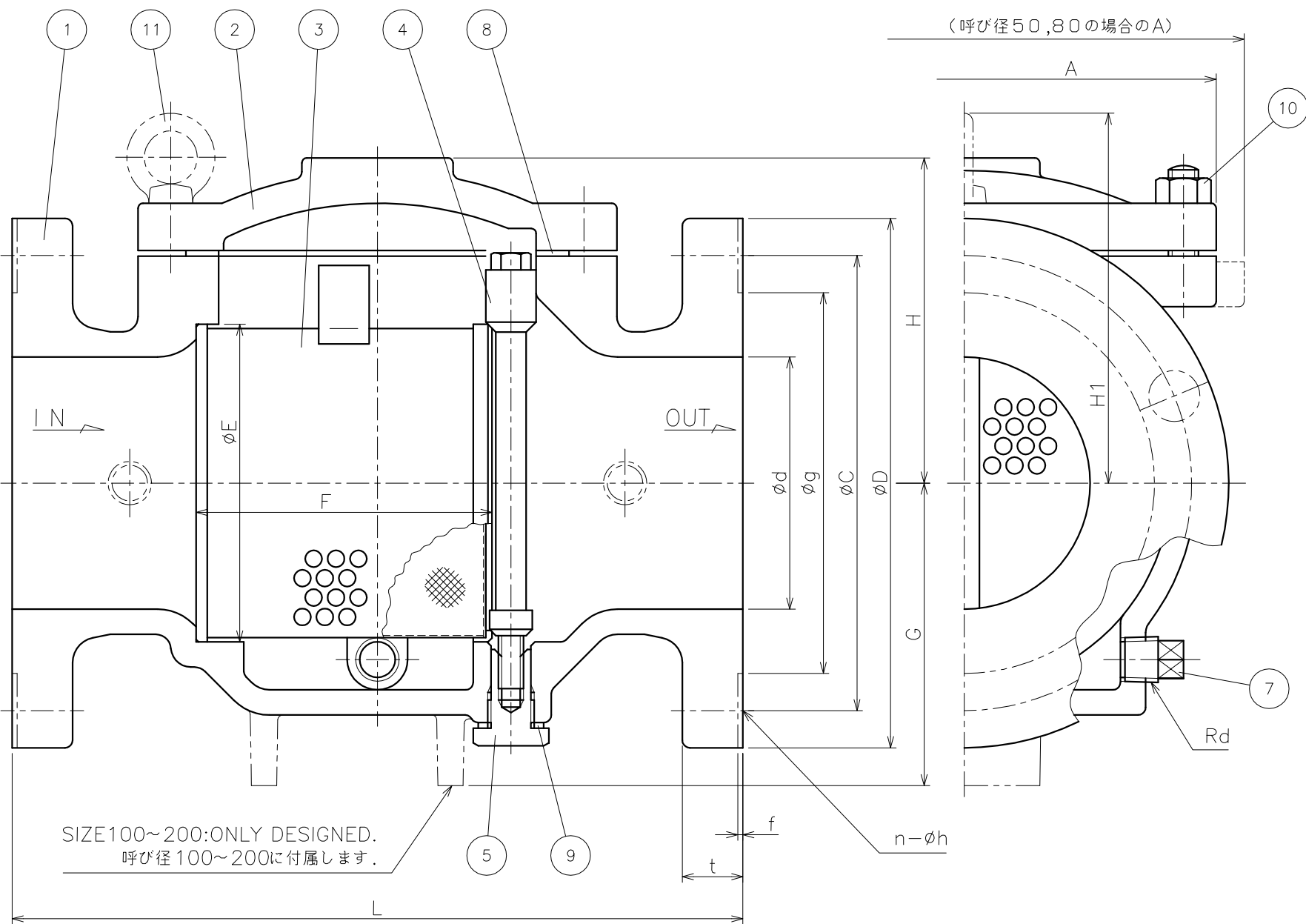
DIMENSIONS (mm) FLANGE CODE: JIS 10K
