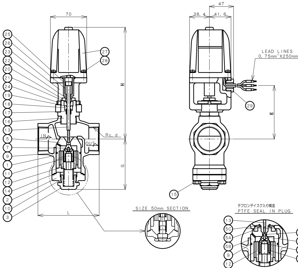
DIMENSIONS (mm)
