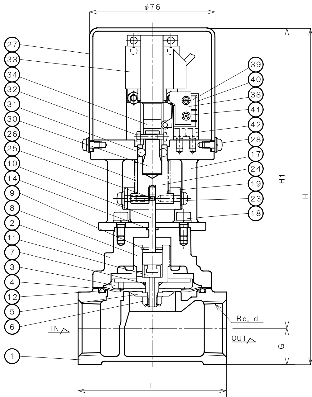
DIMENSIONS (mm)
