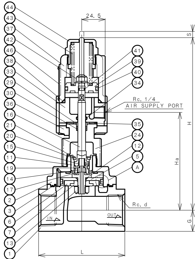
PARTS (A)
