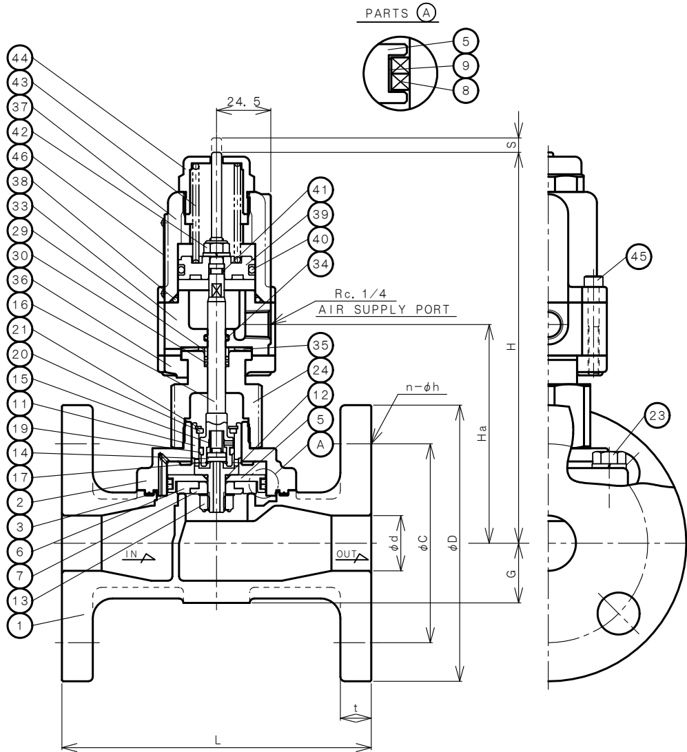
DIMENSIONS (mm) FLANGE CODE: JIS 10K FF
