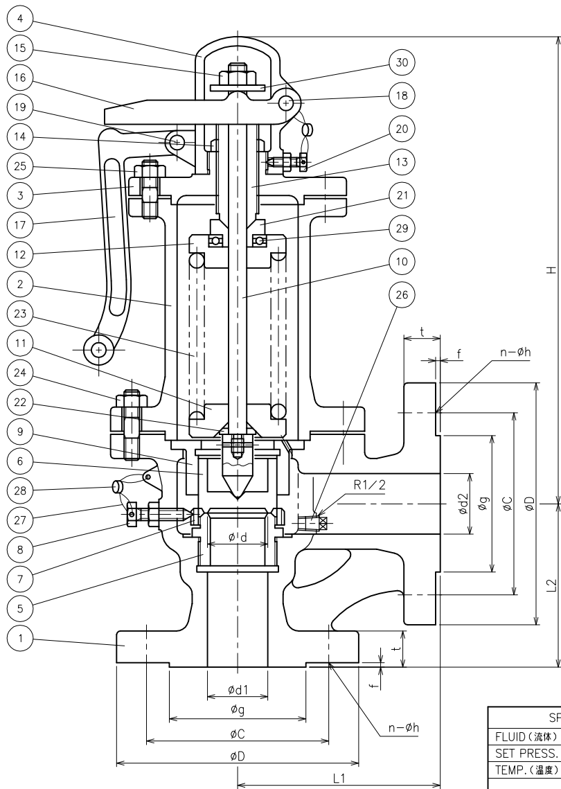
DIMENSIONS (mm)
